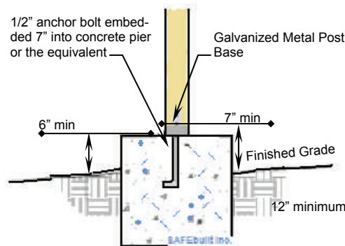
Sample footing detail
